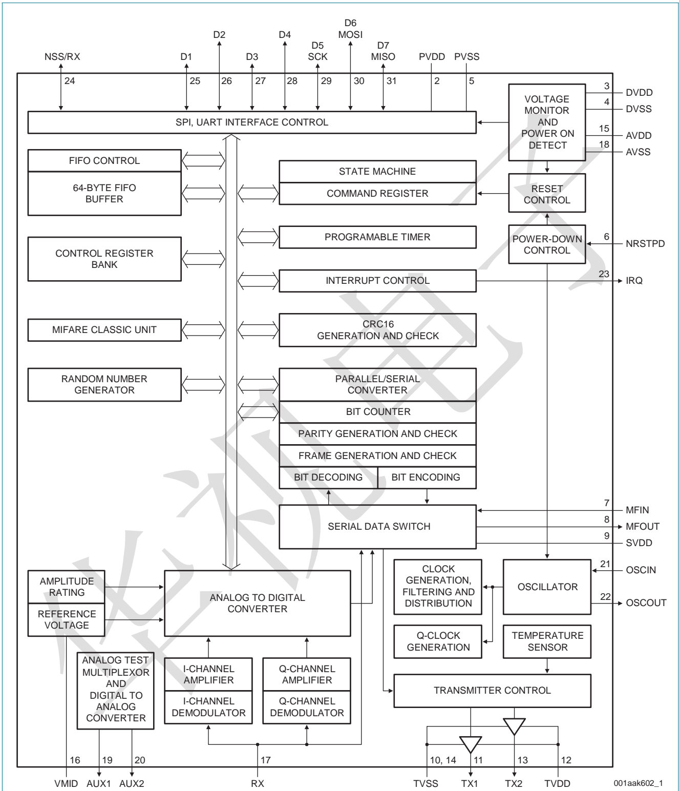
Fig 2. Detailed block diagram of the MF CV520
